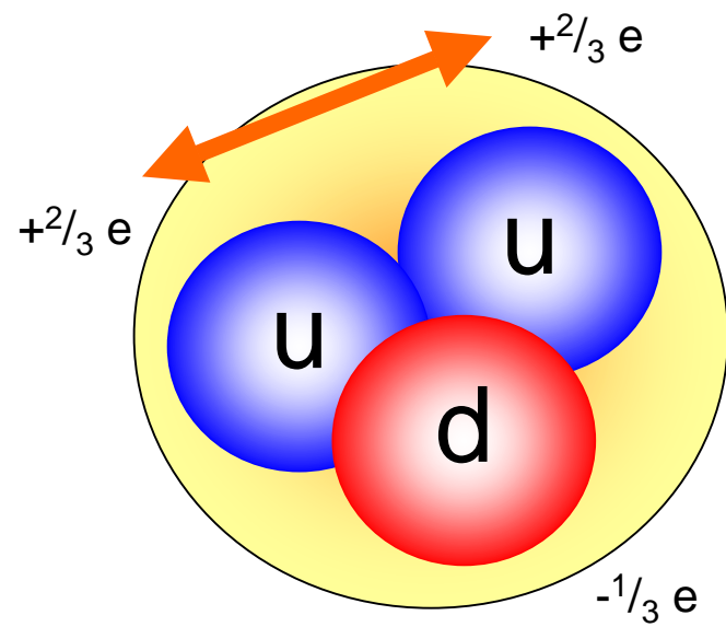
Proton
