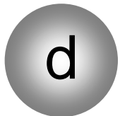
down-Quark
